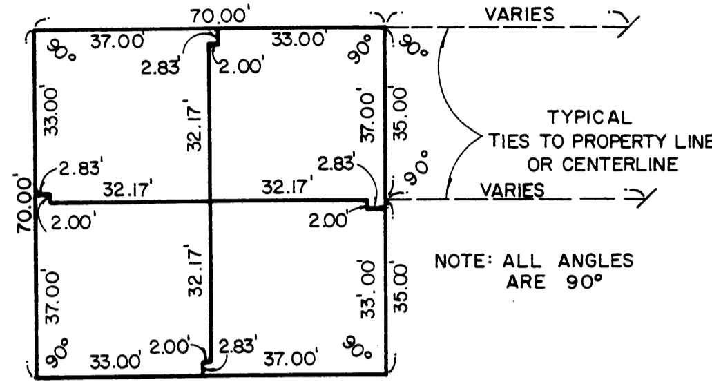
TYPICAL LOT LAYOUT N.T.S.
